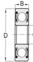
Type -2RS with double seals
